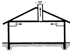
5 Extract ventilation
